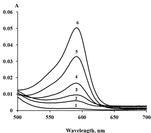
Fig. 1. Absorption spectra of Bromophenol Blue against the background of Phenol Red dye in the spectrophotometric determination of bromide ions in the presence of excess ammonium ions. Bromide concentrations, \mu\text{g L}^{-1} : 1 – 0; 2 – 20; 3 – 50; 4 – 100; 5 – 200; 6 – 300. 1
