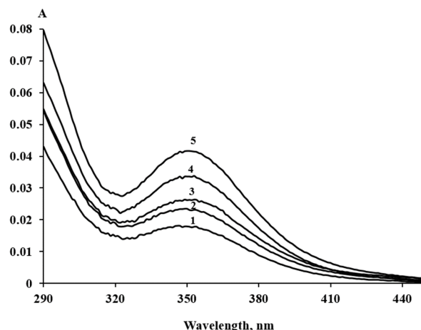
Fig. 3. UV-Vis spectra for the determination of bromide as triiodide ion after solvent extraction of bromine into CHCl_3 . Bromide concentrations, \text{mg L}^{-1} : 1 – 0; 2 – 1; 3 – 2; 4 – 5; 5 – 10.
