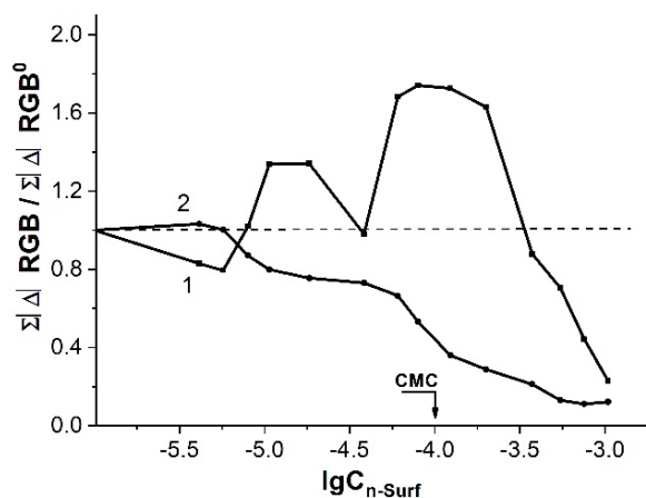
Figure 8. Normalised dependences of the BSA analytical signal on the concentrations of TX-305 (1) and Tween 20 (2). C_{\text{CBBG}}=2.0 \cdot 10^{-5} \text{ M} , C_{\text{BSA}}=5 \text{ mg L}^{-1} , C_{\text{n-Surf}}=4.0 \cdot 10^{-6} \text{--} 1.0 \cdot 10^{-3} \text{ M} , w(\text{EtOH})=5\% \text{ (v/v)} , \text{pH}=1.0 .
