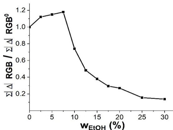
Figure 4. Normalised RGB-signal of BSA in the reaction with CBBG in solution on the ethanol concentration. C_{CBBG}=2.0 \cdot 10^{-5} M, C_{BSA}=5 mg/l, pH=1.0.
