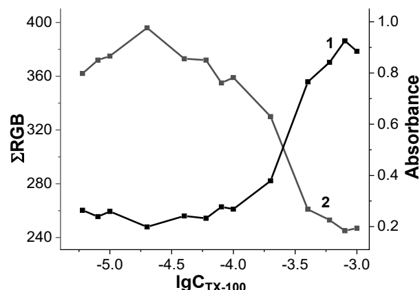
Figure 6. Spectrophotometric (1) and colorimetric (2) signals of CBBG in solution on the TX100 concentration. C_{\text{CBBG}} = 2.0 \cdot 10^{-5} M, C_{\text{TX-100}} = 6.0 \cdot 10^{-6} – 1.0 \cdot 10^{-3} M, \text{pH}=1.0 , \lambda=640 \text{ nm} .
