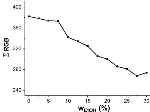
Figure 3. Colorimetric CBBG signal on the EtOH concentration. C_{CBBG}=2.0 \cdot 10^{-5} M, pH=1.0.
