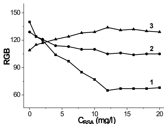
Figure 2. Colorimetric signal R(1), G(2), B(3) of CBBG–BSA aqueous solutions. C_{CBBG}=2.0 \cdot 10^{-5} M, pH=1.0.
