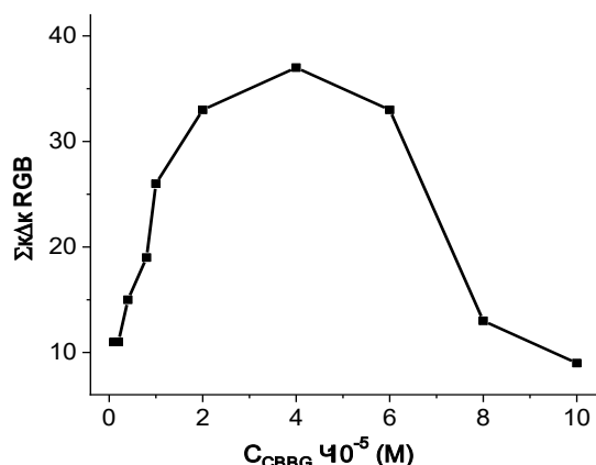
Figure 5. Colorimetric signal of BSA in the reaction with CBBG on the reagent concentration. C_{\text{BSA}} = 5 \text{ mg L}^{-1} , w(\text{EtOH}) = 5\% (v/v), \text{pH}=1.0 .
