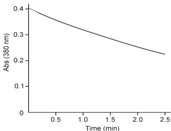
Fig. 4. Decomposition of PTA-SO over 2,5 min. c(\text{PTA}) = 1.0 \times 10^{-4} \text{ M} , c(\text{HCl}) = 6.0 \times 10^{-3} \text{ M} , c(\text{KHSO}_5) = 0.005 \text{ M} .
