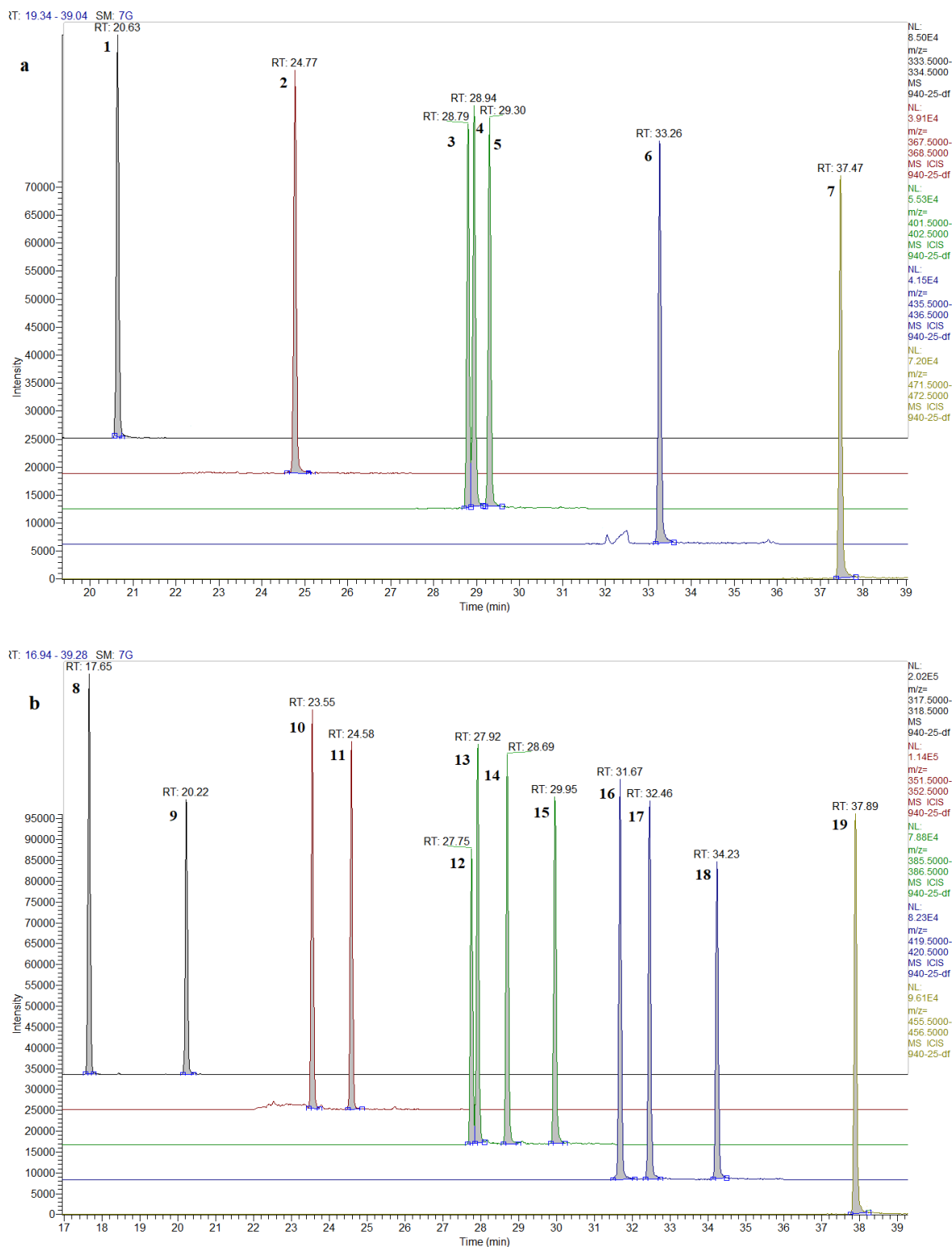
Fig. 5. Chromatographic separation of the most toxic PCDD/Fs congeners ( 1 \text{ ng mL}^{-1} for octasubstituted compounds and 0.5 \text{ ng mL}^{-1} for others): a – peak identification: (1) 2,3,7,8-TCDD; (2) 1,2,3,7,8-PeCDD; (3) 123478-HxCDD; (4) 123678-HxCDD; (5) 123789-HxCDD; (6) 1,2,3,4,6,7,8-HpCDD; (7) OCDD; b – peak identification: (8) 1368-TCDF (Recovery standard); (9) 2,3,7,8-TCDF; (10) 12378-PeCDF; (11) 23478-PeCDF; (12) 123478-HxCDF; (13) 123678-HxCDF; (14) 234678-HxCDF; (15) 123789-HxCDF; (16) 1234678-HpCDF; (17) 1234689-HpCDF (Recovery standard); (18) 1234789-HpCDF; (19) OCDF.
