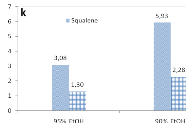
Figure 3. SiO 2 -C18. The dependence of retention factors (k) of squalene and tocopheryl acetate on the ethanol content in the mobile phase.
