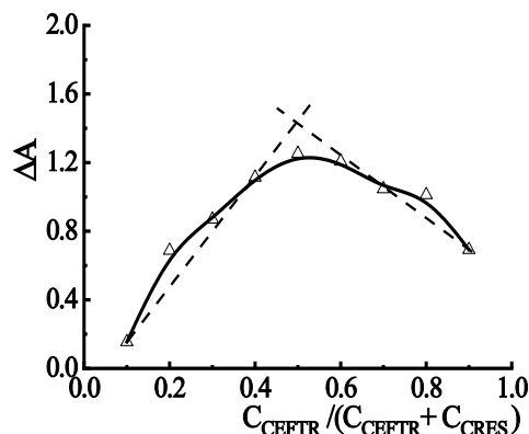
Fig.4. The continuous variation curve for the azo compound of diazotized ceftriaxone and CRES. C_{\text{CEFTR}+\text{CCRES}} = 3.7 \cdot 10^{-4} M. Diazotization conditions: C_{\text{HCl}} = 12.0 M (initial conc., V = 0.5 mL), C_{\text{NaNO}_2} = 1.0 \cdot 10^{-3} M, t_{\text{diazot.}} = 5 min. Conditions for azo coupling: C_{\text{NaOH}} = 0.16 M; \lambda_{\text{max}} = 516 nm, l = 1 cm.
