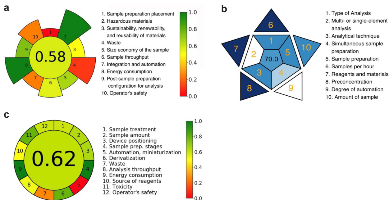
Fig. 6. Generic result of assessment of the developed spectrophotometric procedure for the determination of ceftriaxone using o -cresol: a) AGREEprep; b) BAGI; c) AGREE metric.
