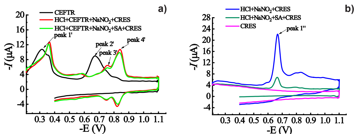
Fig. 5. Cyclic voltammograms of solutions of CEFTR azo coupling products with CRES. \nu = 2.5 \text{ V} \cdot \text{s}^{-1} . Diazotization conditions: C_{\text{HCl}} = 12.0 M (initial conc., V = 0.5 mL), C_{\text{CEFTR}} = 7.5 \cdot 10^{-5} M, C_{\text{NaNO}_2} = 7.5 \cdot 10^{-4} M, C_{\text{SA}} = 1.1 \cdot 10^{-4} M. Conditions for azo coupling: C_{\text{CRES}} = 7.5 \cdot 10^{-4} M, C_{\text{NaOH}} = 0.16 M.
