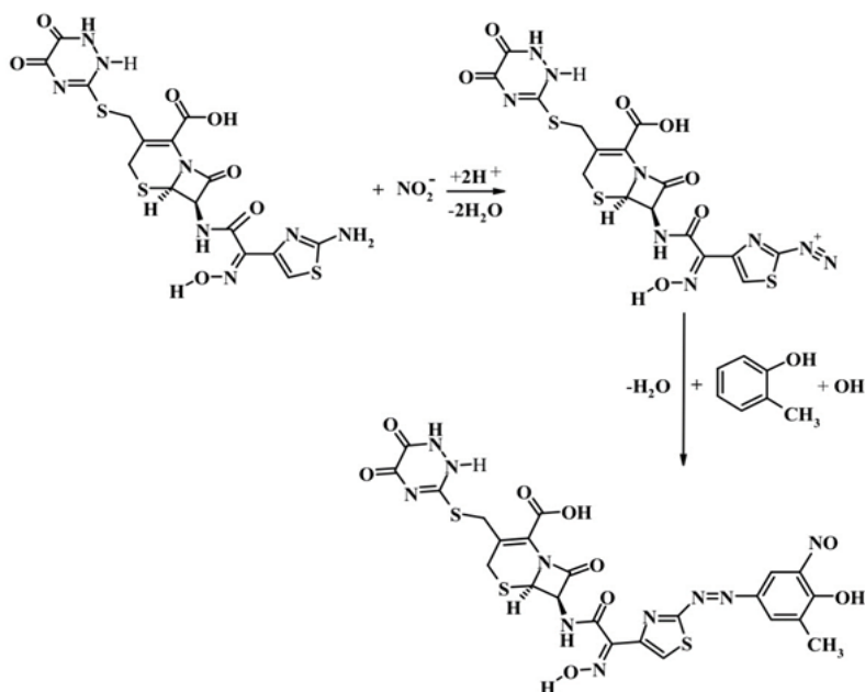
Scheme 1. Scheme of ceftriaxone interaction with o -cresol.
