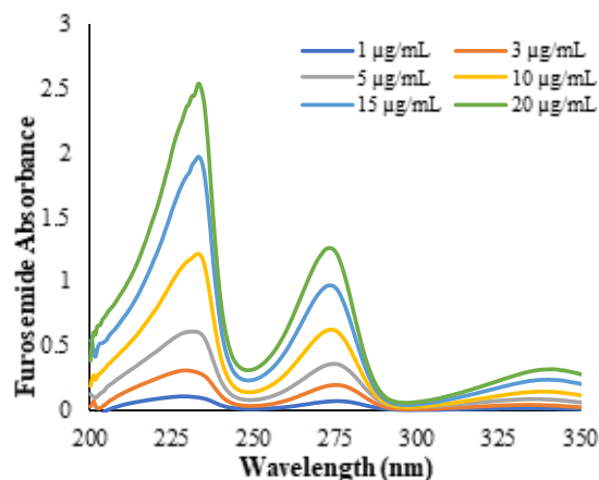
Figure 5: FUR absorbance vs. wavelength
