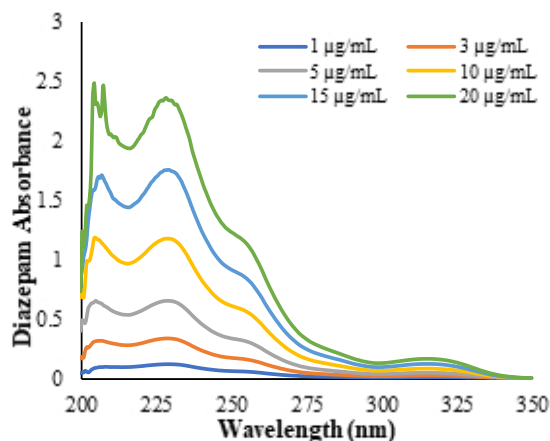
Figure 4: DIA absorbance vs. wavelength
